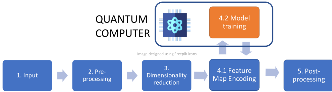
Fig. 8: Hybrid Quantum-Classical Machine Learning Workflow.
