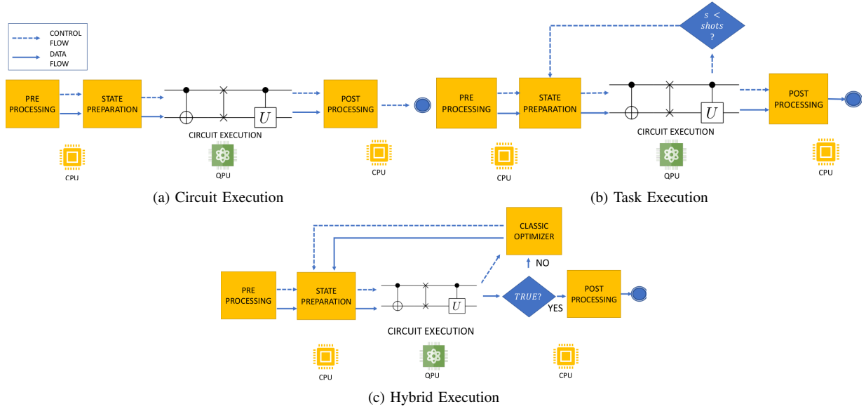
Fig. 2: Hybrid Execution Models, from [5].
