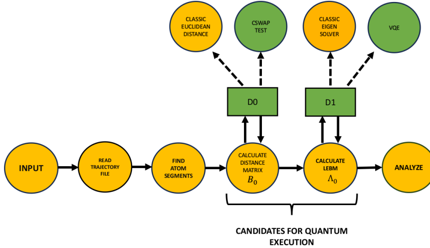
Fig. 1: A Hybrid Quantum-Classical Workflow, from [5].
