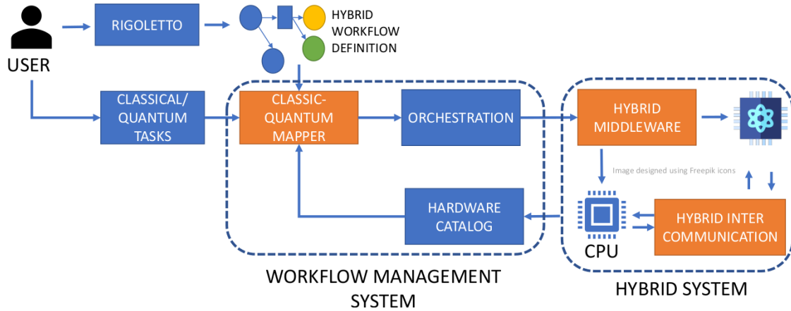
Fig. 3: Usage of RIGOLETTO within Hybrid Quantum-Classical WMS.
