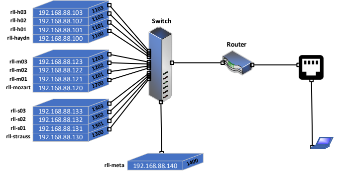
Fig. 1. System Configuration of the RUCON LiveLab.
