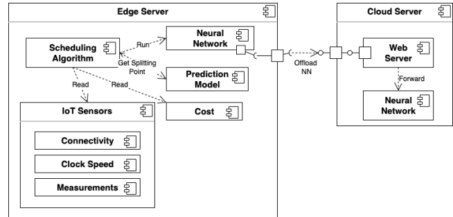
Figure 2: UML Component Diagram of the Proposed System.
